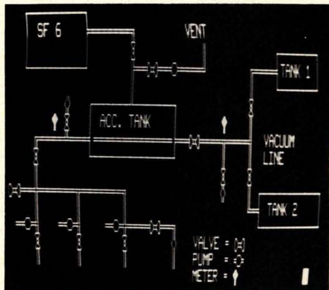
Photo 2: A piping diagram, an example of what can be done with the programmable character generator.
