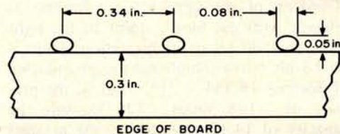
Figure 3: Size and spacing of Molex connector slots relative to lower board edge.
