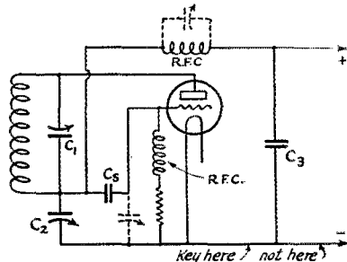
FIG. 5. THE FEEDBACK-CONTROL CONDENSER MAY BE USED IN SEVERAL WAYS
