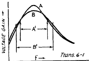
FIG. 4. RESULT OF INSUFFICIENT GRID BIAS IN BROADENING A PEAKED TRANSFORMER
