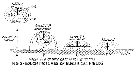
FIG. 3—ROUGH PICTURES OF ELECTRICAL FIELDS.
