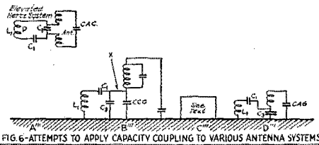
FIG. 6-ATTEMPTS TO APPLY CAPACITY COUPLING TO VARIOUS ANTENNA SYSTEMS
