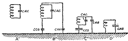
FIG. 5-DISTRIBUTED CAPACITIES LUMPED
