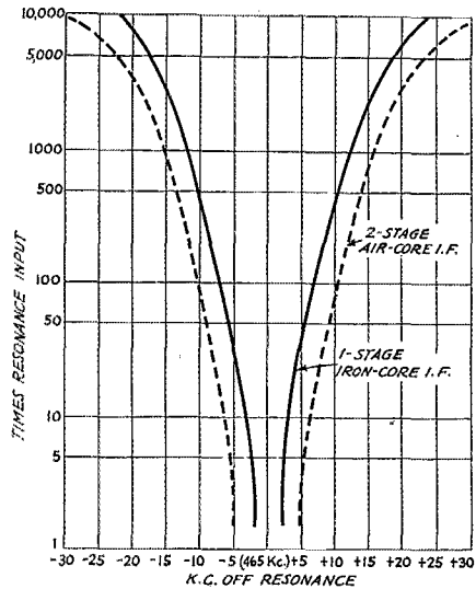
FIG. 3.—SELECTIVITY CURVES FOR THE TWO I.F. AMPLIFIERS, WITH THE CRYSTAL SHORTED OUT, SHOWING THE IMPROVEMENT ACCOMPLISHED IN THE SINGLE-STAGE ARRANGEMENT WITH THE MORE EFFICIENT CRYSTAL FILTER CIRCUIT AND IRON-CORE TRANSFORMERS
