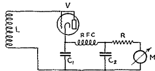
FIG. 1—CIRCUIT OF THE SIMPLE DIODE-TYPE CARRIER-SHIFT INDICATOR WHICH CONSTITUTES "MEANS TO INSURE THAT THE TRANSMITTER IS NOT MODULATED IN EXCESS OF ITS MODULATION CAPABILITY," IN ACCORDANCE WITH THE NEW REGULATIONS
