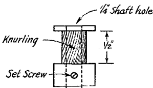
FIG. 3—DETAIL OF TAPE PULLER
