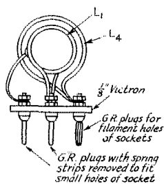
Input coil connections on six-pin socket
