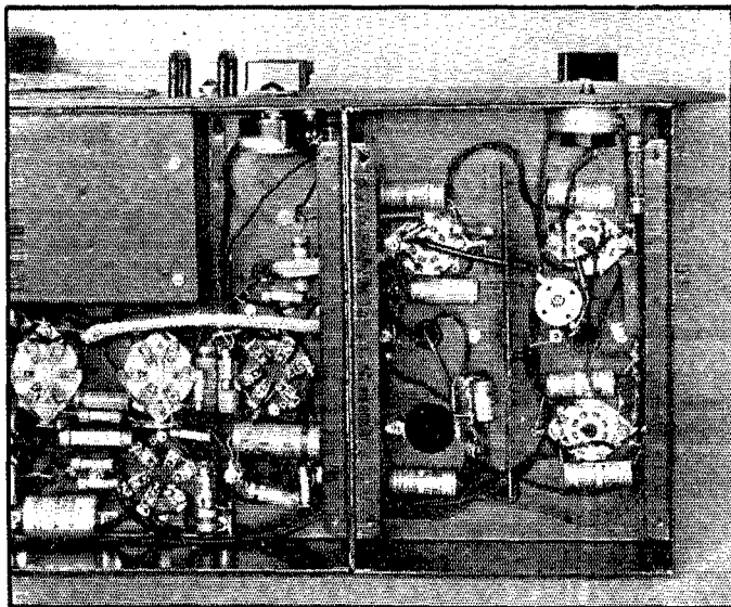
THE SIMPLE CIRCUIT OF THE SILENCER UNIT SEPARATES THE INPUT TRANSFORMER AND 6L7 CIRCUITS FROM THE NOISE AMPLIFIER-RECTIFIER.
