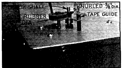
FIG. 2—TAPE PULLER SHOWING KNURLED BRASS SHAFT AND RUBBER WHEEL AND TAPE GUIDE
