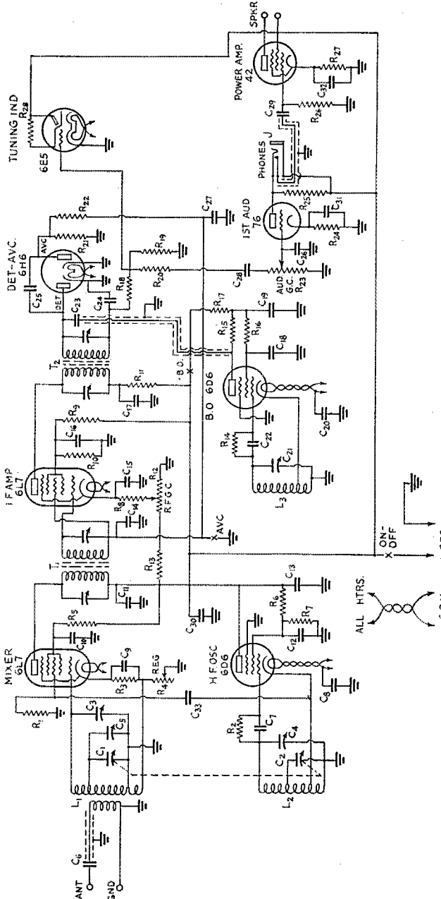
FIG. 1—THE RECEIVER CIRCUIT DIAGRAM
