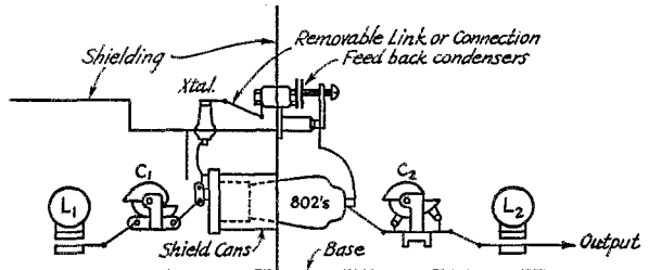
FIG. 4—SUGGESTED PHYSICAL LAYOUT FOR TRANSMITTER COMPONENTS TO AVOID FEEDBACK
