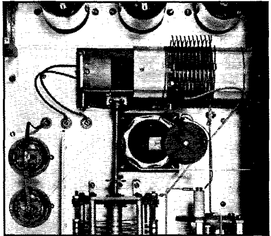
ANOTHER INSTALLATION OF INDUCTIVE NEUTRALIZATION
