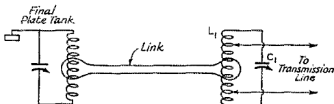
FIG. 4—THE ANTENNA COUPLING CIRCUIT USED AT WIJPE
