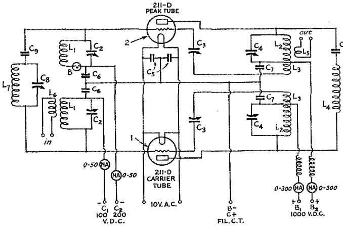
FIG. 5—THE FINAL CIRCUIT FOR 3950-KC. OPERATION
