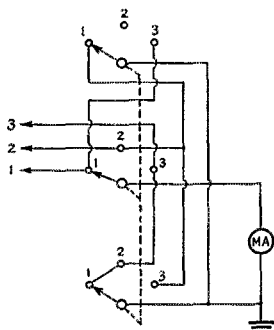
FIG. 2.—A METER-SWITCHING CIRCUIT FOR HANDLING THREE STAGES
