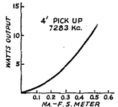
FIG. 5—FIELD STRENGTH METER CALIBRATION AT 7283 KC., 4-FOOT PICK-UP ANTENNA
