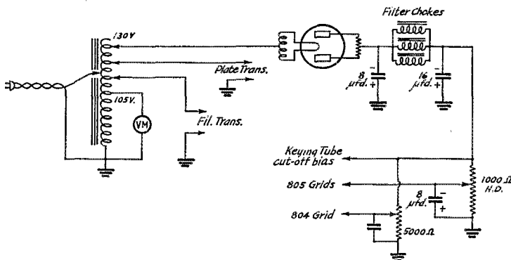
FIG. 4—USING THE AUTO-TRANSFORMER TO PROVIDE "C" BIAS FOR THE TRANSMITTER
