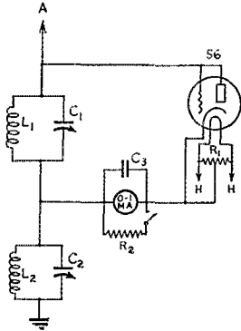
FIG. 1—SCHEMATIC CIRCUIT OF THE SIMPLE FIELD-STRENGTH METER USED IN DETERMINING HARMONIC RADIATION
