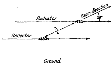
FIG. 2—ARRANGEMENT OF ANTENNA AND REFLECTOR FOR CONCENTRATING RADIATION IN ONE DIRECTION
