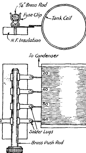
FIG. 6—AN EASILY-CONSTRUCTED SHORTING SWITCH FOR BAND-CHANGING
