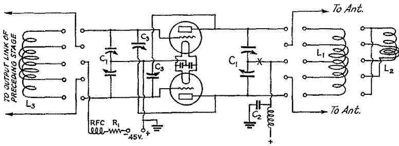
FIG. 3—COMPLETE CIRCUIT OF THE 808 AMPLIFIER
