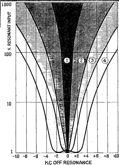
Chart showing the variations in selectivity obtainable with Sky-ride 23 Wide Range Variable Selectivity.
