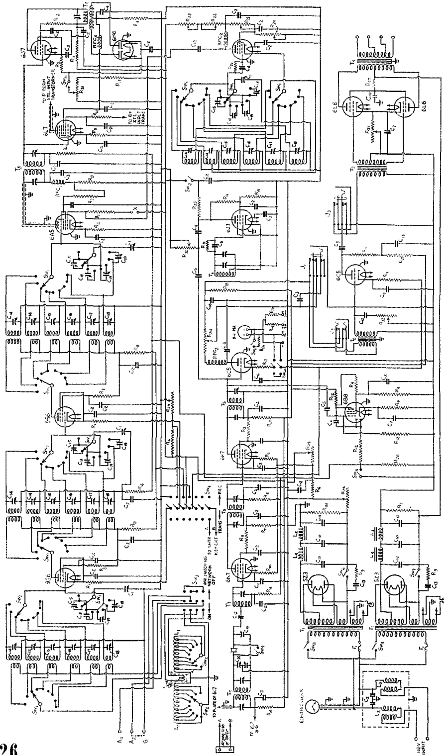
Fig. 1 — The receiver circuit diagram. C 1 — 4-section ganged condenser, 175 \mu fd. per section, and dial (National PW-4). C 2 — 0.1- \mu fd., 600-volt tubular paper. C 3 — 0.25- \mu fd., 600-volt tubular paper. C 4 — 100- \mu fd. mica. C 5 — 0.001- \mu fd. mica. C 6 — 25- \mu fd., 50-volt electrolytic. C 7 — 25- \mu fd., 100-volt electrolytic. C 8 — 0.005- \mu fd. mica.
