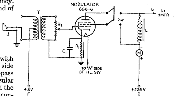
Fig. 4 — Modulator wiring diagram. C 1 — 25- \mu fd., 25-volt electrolytic. R 1 — 600 ohms, 1-watt. R 2 — 0.5-megohm potentiometer. J — Open circuit jack. T — D.b. mike to single-grid transformer (Stancor A-4708). L — Filter choke used as modulation choke (Stancor C-1002) (30 henrys, 50 ma., 400 ohms d.c. resistance). Sw — D.p.d.t. toggle switch. M — 0-50 milliammeter (Triplett).
