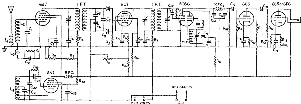
Fig. 1 — Wiring diagram of the six-tube superhet.
