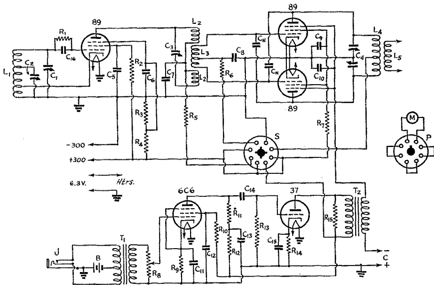
Fig. 1 — Circuit diagram of the low-cost 5-meter transmitter.
