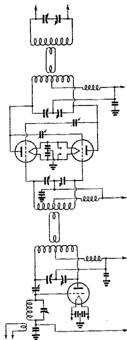
Fig. 1—General circuit of the transmitter. Coil taps are not shown in this diagram. Aside from the high voltage connections to the tuning condenser rotors, the circuits are completely conventional. Link coupled buffer, link coupled push-pull amplifier, and link coupled antenna tuner are used for ease of obtaining correct match and loading throughout.
