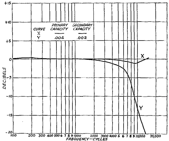
Fig. 6 — Frequency characteristic of the transformer alone (X) and with capacities across primary and secondary (Y). Curve Y corresponds to curve H in Fig. 5.
