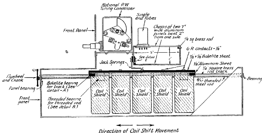
SIDE ELEVATION
