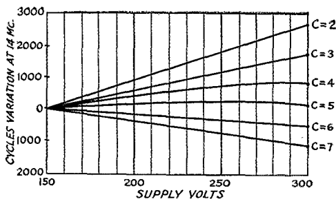
Fig. 2—Showing the variation of frequency with plate voltage for various positions of the cathode tap.
