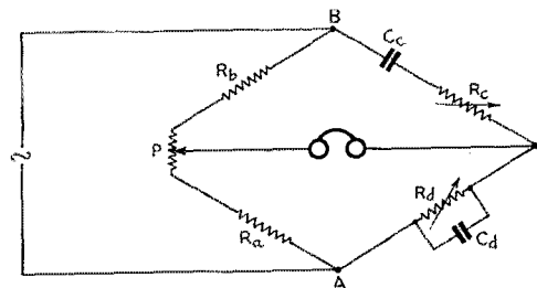
Fig. 1 — Fundamental Wien bridge circuit.
