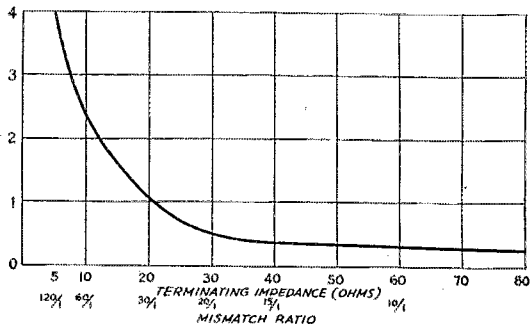
Fig. 1 — An experimentally-determined curve of the line loss in a 1\frac{1}{2} wavelength long 600-ohm line with various degrees of mismatch.
