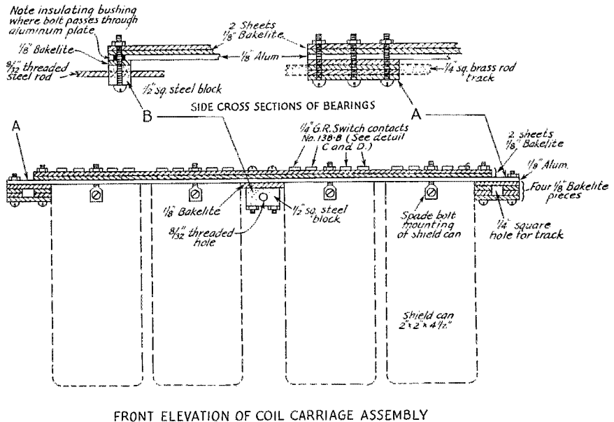
Fig. 2—Details of construction of coil unit and the sleeves which fit the brass-rod tracks. The threaded arrangement for moving the unit is also shown in detail.
