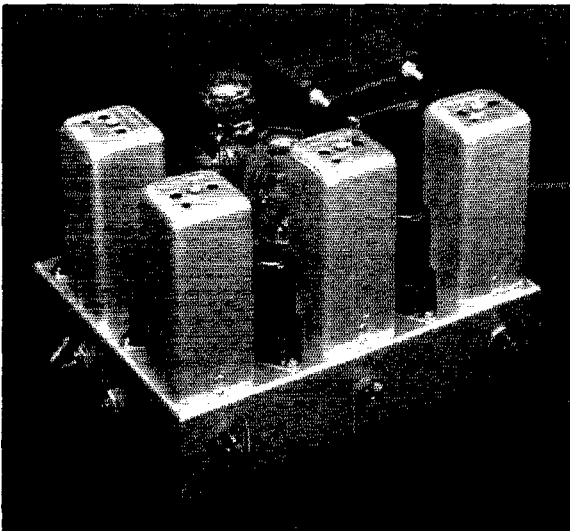
The 5-Mc. f.m./a.m. amplifier is built, complete with power supply, on a 7-inch by 9-inch by 2-inch chassis. Controls on the front, from left to right, are audio volume control, B-plus switch and limiter control. The switch on the side is for changing from f.m. to a.m. and back, and the jack allows a meter to be plugged in to read limiter current.
