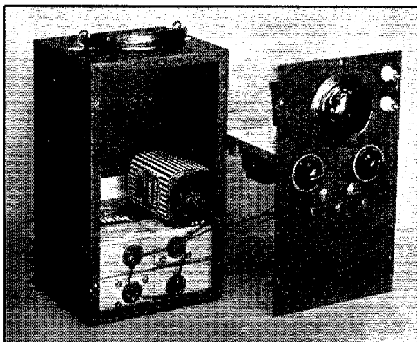
◆ A front view of the transceiver panel layout and the battery compartment. The antenna is a half-wave rod; the upper of the two insulators is only a support. ◆
