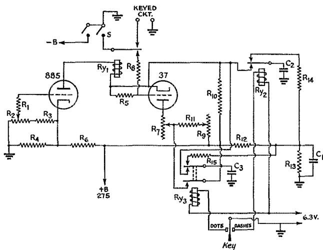
Fig. 8 — Circuit using a.c. relays for dot and dash controls. Values are the same as in Fig. 6 with the following exceptions: C 2 — 1- \mu f. 400-volt paper. R 15 — 100 ohms, 1-watt. Ry 2 , Ry 3 — 6-volt a.c. relay, d.p.d.t. (Ward Leonard 507-505).
