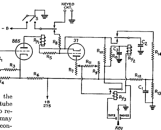
Fig. 6 — Circuit diagram of the electronic key shown in the photographs.
