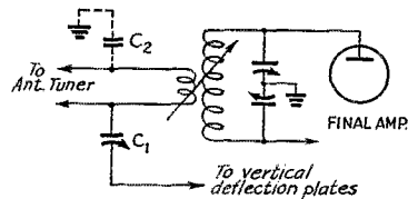
Fig. 4 — Coupling oscilloscope to link output. (See text for values.)
