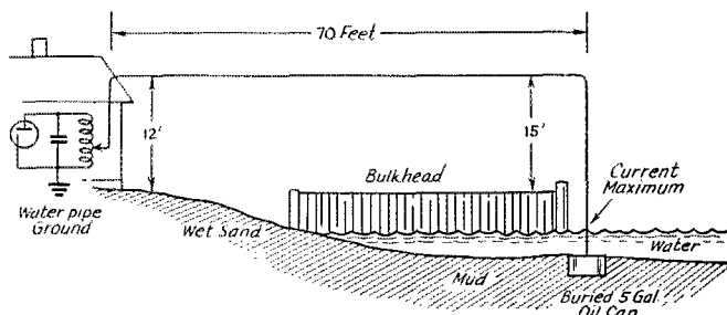
Fig. 3 — Shore location and antenna of WIANC/1 at Grove Beach Point, 1938 B.H. (before hurricane).
