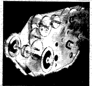
New type inertia-controlled back-lash-free dial mechanism on both main tuning and bandsread dials. This mechanism is preloaded and the main shafts are supported at both ends with ball bearings.
