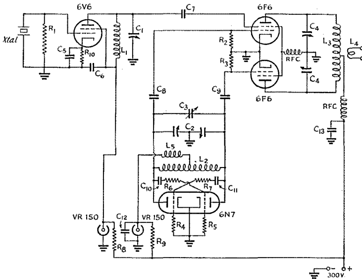
Fig. 1 — Heterodyne exciter circuit
