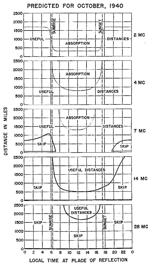
Fig. 1. Useful distances for radio wave propagation via the regular layers of the ionosphere, predicted for October, 1940. The 56-Mc. band will be useful only for local transmission (optical and quasi-optical paths).
