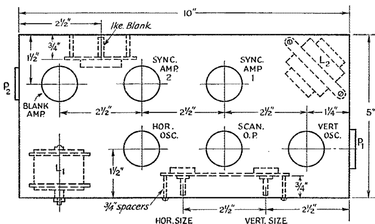
Chassis depth = 3" Socket holes 1/8" diam.
