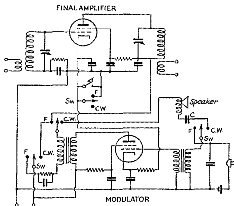
Fig. 3 — W9EHC's scheme for converting modulator in portable to keying-monitor oscillator for code work. The four switches are sections of a four-gang switch. The size of the capacity C determines the pitch of the audio tone generated.
