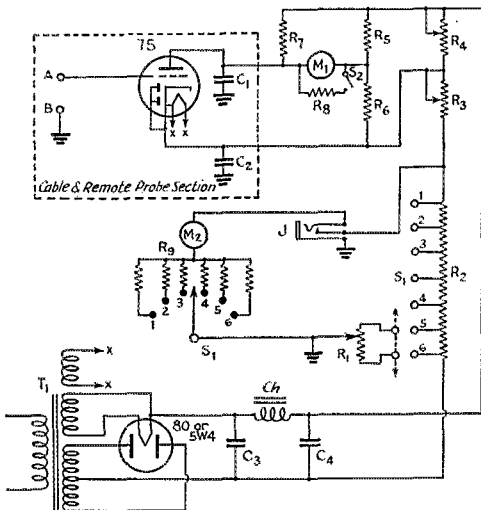
Fig. 4 — The practical v.t.v.m. circuit.
