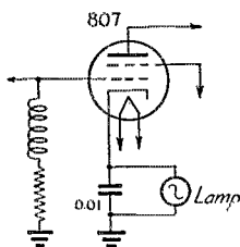
Fig. 5—Cathode lamp for protecting 807 as used by W9BPS.
