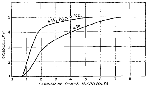
Fig. 5 — Readability comparison of a frequency-modulation system and its equivalent amplitude-modulation system. Maximum frequency deviation = 6 kilocycles. Audio band = 5 kilocycles.
