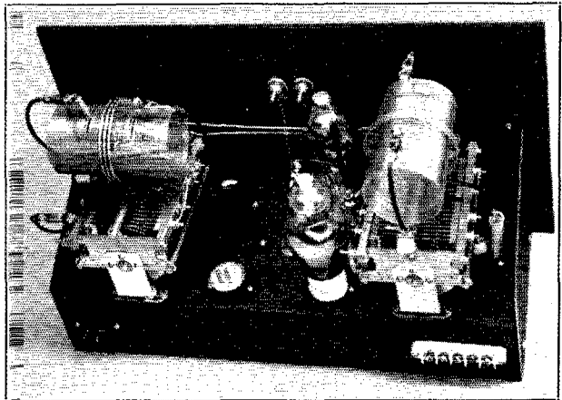
Rear view of two-band transmitter. The chassis is 7 inches by 3 inches by 17 inches. The plate tank is to the right and the antenna tuner to the left. The two neutralizing condensers are centrally located between the two tubes.
