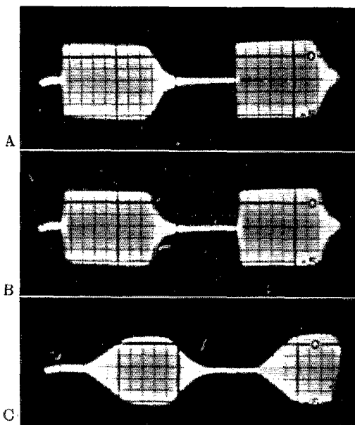
Fig. 5 — Oscilloscope waveforms of oscillator keying using complete key filters.
