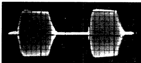
Fig. 7 — Negative power lead keying of amplifier with optimum key filter. The amplifier operated at 70 ma. at 400 volts, and the filter was the primary of a small filament transformer and 0.5 \mu fd. There is slightly more lag on make than necessary.
