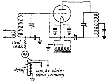
Fig. 6 — WILRU's scheme for push-to-talk without fixed bias. The relay used is the Utah R.A.C. 110. Connected in the grid return circuit of the buffer stage, the relay opens the primaries of the plate transformers which supply the amplifier stages when excitation is removed.
