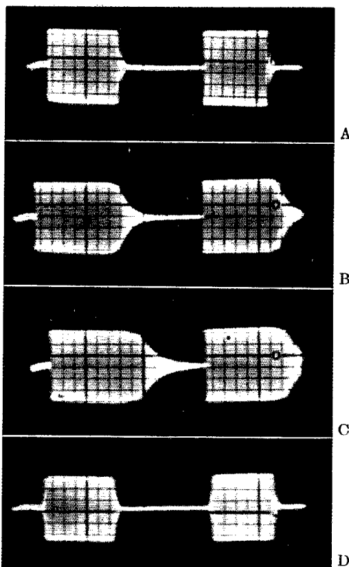
Fig. 4 — A group of oscillograms of a self-excited oscillator keyed in the negative power lead. The oscillator draws 2.8 ma. at 150 volts and is followed by two Class-A amplifier stages. The left-hand side of the character is "make," and the right-hand side is "break." The black lines are part of the 'scope face.
