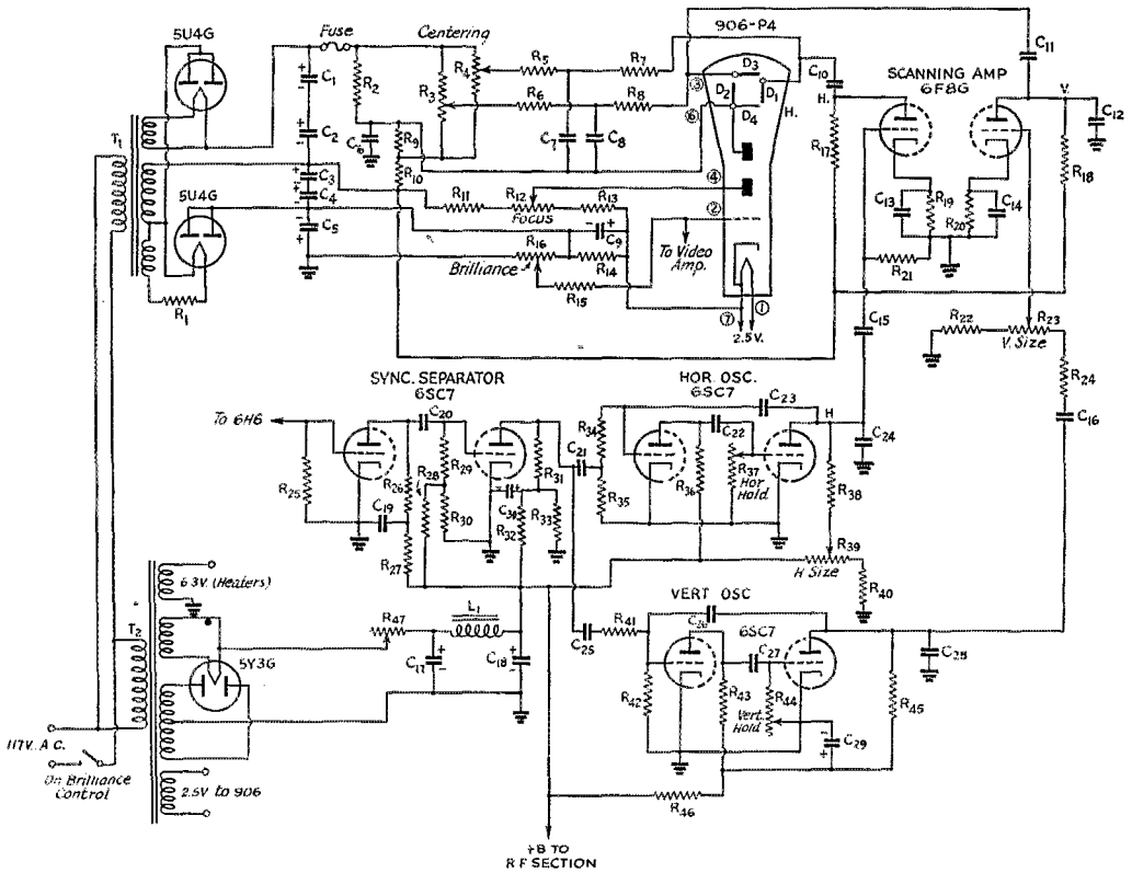
Fig. 3 — Scanning and Kinescope circuits with power supplies.
