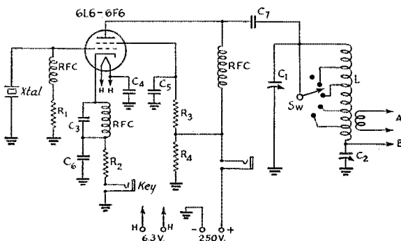
Fig. 1 — Wiring diagram of the portable transmitter.
