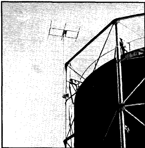
How does he get away with it? W9CNJ, Robinson, Ill., has his 3-element "Q" array mounted at the top of a gas storage tank, 95 feet above ground. Rotating device is a revamped chain hoist. Photograph by W9BDL and W9GTS.
