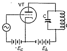
Fig. 4 — In this circuit, if the grid-plate transconductance of VT is negative, the r.f. voltage across the LC tank will be in phase with the signal voltage at the grid. To convert the circuit to an oscillator, all that is necessary is to capacitively couple the grid and plate and replace the generator by a grid-leak. Such an oscillator is called a transitron oscillator.
