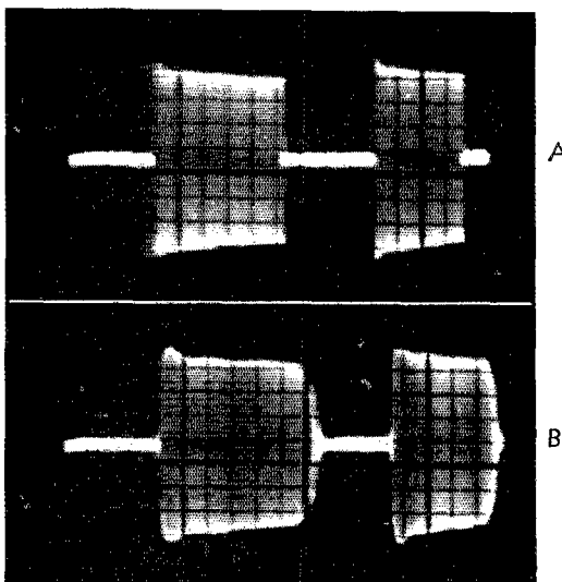
Fig. 7—Grid-block keying of an amplifier. A shows the characteristic with only the normal grid leak and r.f. by-pass condenser, B shows the addition of 0.1 \mu fd. across the condenser. The clicks of B were very slight, with almost none at all on "break." Note that the addition of capacity in B has made the dots "heavier," requiring a slight readjustment of the key if a bug is used.
