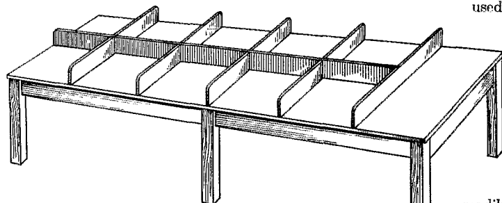
Fig. 3 — A suggested form of construction for the code-instruction table. Dimensions may be varied to suit individual club needs. Legs may be made of 4 by 4 stock; top and side rails of 1-inch boards. Appropriate bracing should be provided underneath. A coat or two of shellac after the table is finished will prevent shrinkage.
