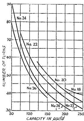
Fig. 1 — Turns required for various tuning capacities to resonate at 1700 kc. Sizes of enameled wire are indicated on the curves. Coils close-wound on 1\frac{1}{2} -inch forms.
