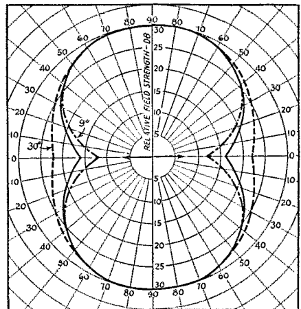
Fig. 6 — Directive patterns of a horizontal half-wave antenna at three vertical angles, 9, 15 (solid line) and 30 degrees. The direction of the antenna is indicated by the arrow. These patterns are plotted to a 30-db. scale, which is about proportional to signal strength as determined by ear. If 30 db. represents an S9 signal, 0 on the scale will be about S1. All three patterns are plotted to the same maximum, but actual amplitudes at the various angles will depend upon the antenna height. The patterns show only the shape of the directive pattern as the angle is varied.
