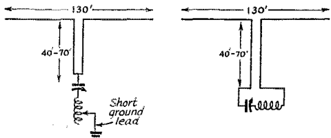
Fig. 6 — Modifications of the center-fed 80-meter antenna for 160-meter operation.
