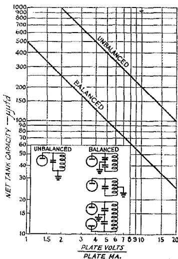
Fig. 3 — Tank capacity required for a Q of 12 for various plate-voltage/plate-current ratios.
