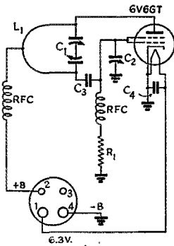
Fig. 1 — Oscillator circuit diagram.
