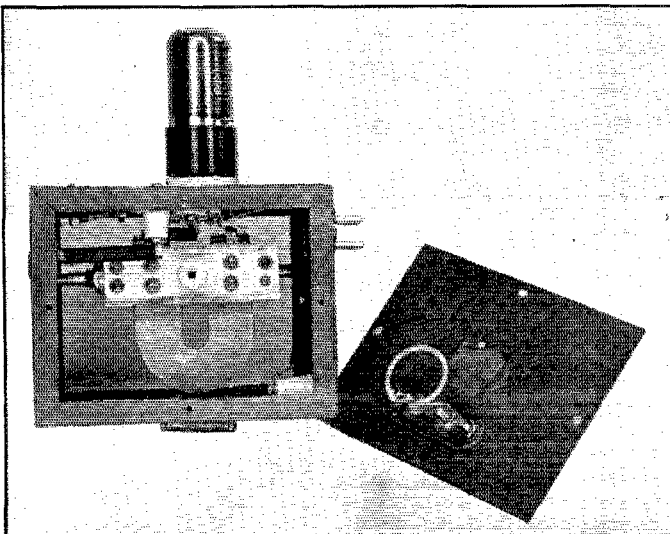
Looking into the oscillator from the antenna-terminal side. The grid choke is in the upper left corner, with its "hot" end supported by a small ceramic stand-off. The plate choke is partly visible in the lower right corner; it is mounted endwise on a ceramic stand-off. The 1-turn antenna coil can be seen mounted on the antenna terminals.
